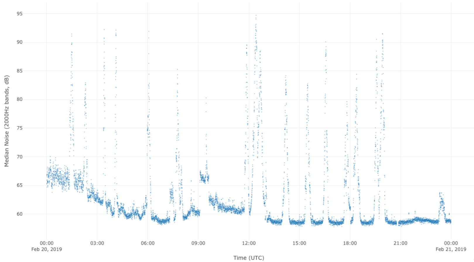
Noise Over Time for 20 February 2019
