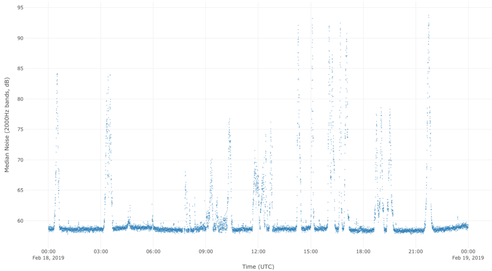
Noise Over Time for 18 February 2019
