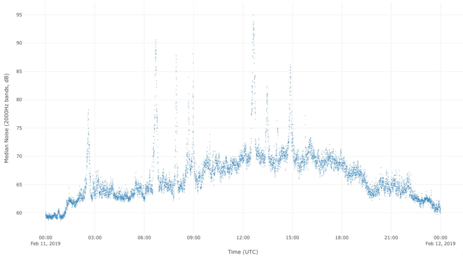
Noise Over Time for 11 February 2019
